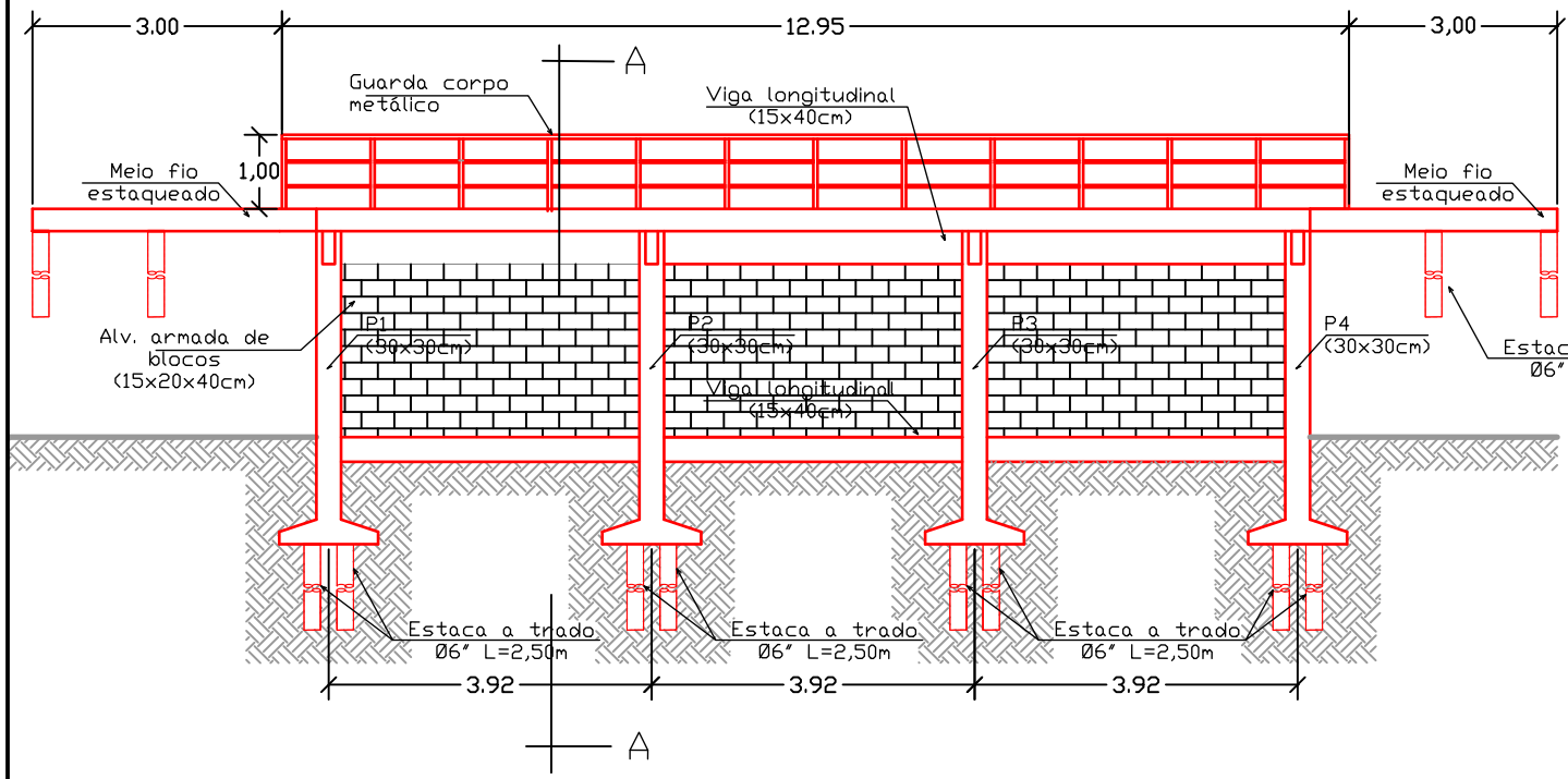
VISTA FRONTAL
